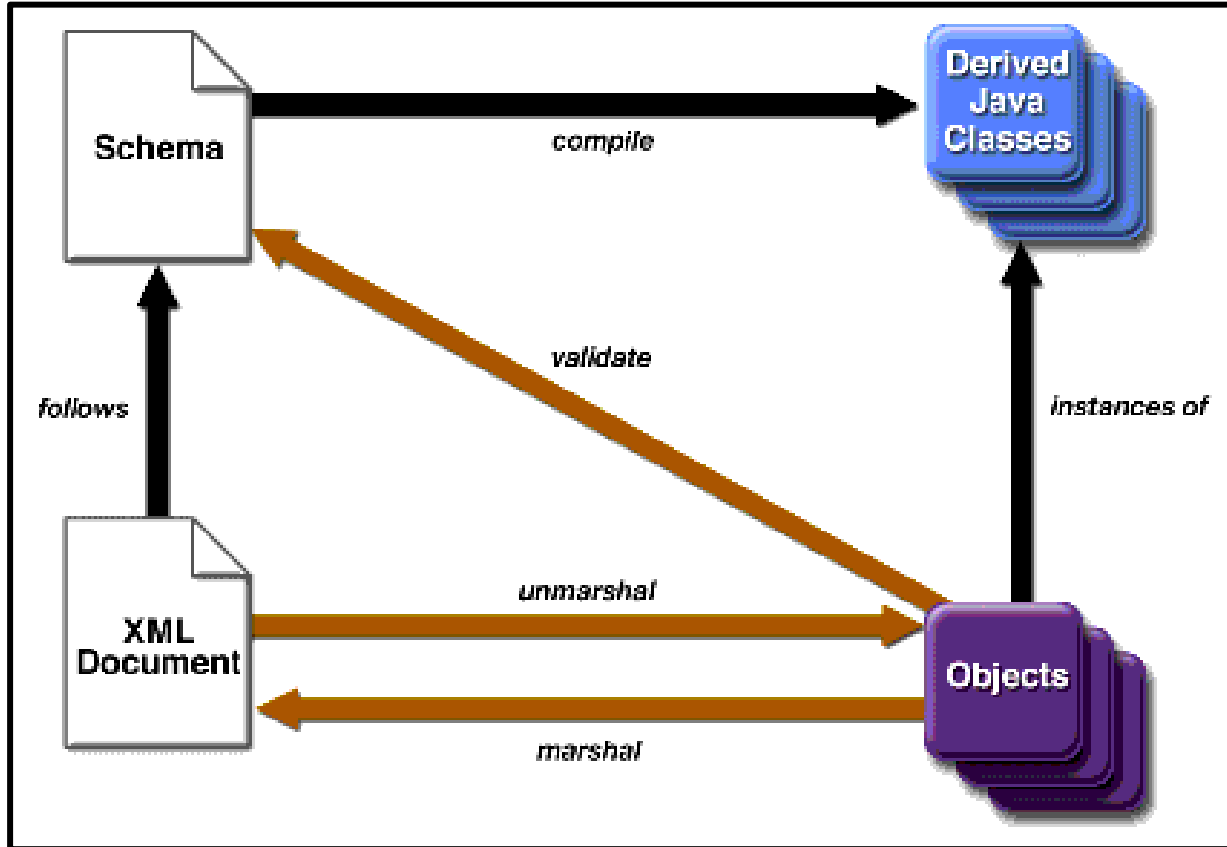
XML-OOP data binding
