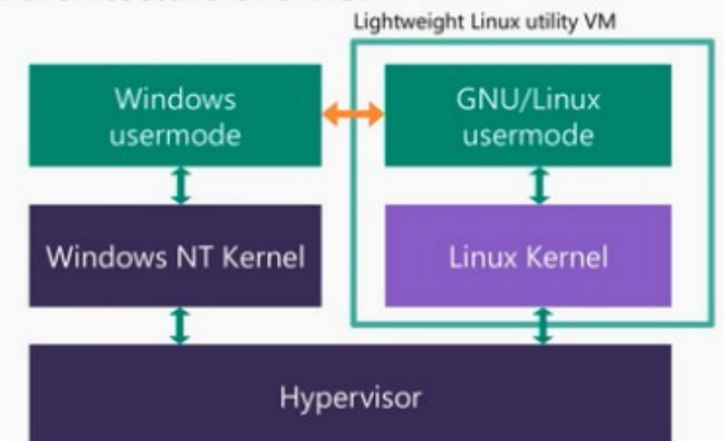
WSL 2 architecture overview
